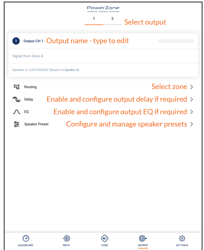
Diagram 5d Output Tab display
