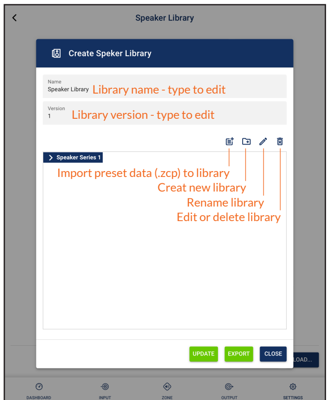
Diagram 5j Speaker Library Creation and Management
