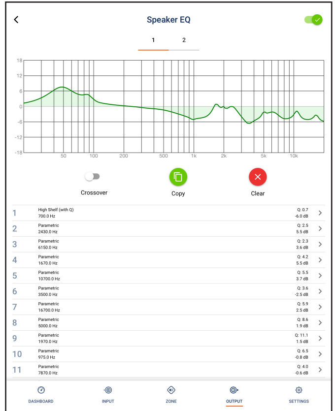
Diagram 5h Speaker Preset parameter adjustment
