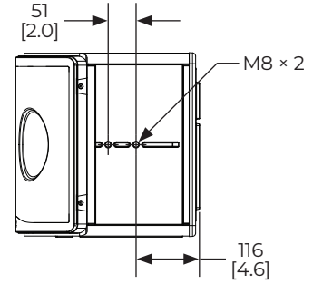
Side View 7
